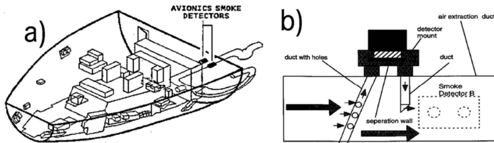
Fig. 2: a) Sketch of an aircraft avionics compartment, b) Installation of duct type smoke detector in Airbus
